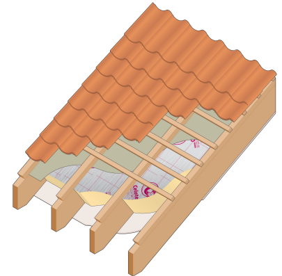
Celotex XR3000 between rafters
